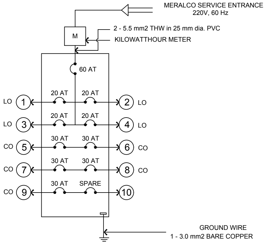
RISER DIAGRAM
