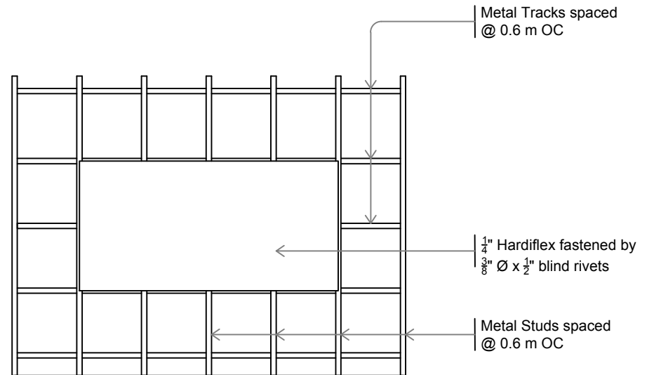
TYPICAL DOUBLE WALL DETAIL SCALE 1 : 50
